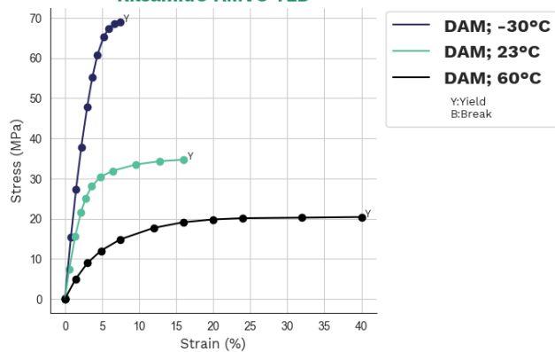
Stress-strain Rilsamid® AMVO TLD
