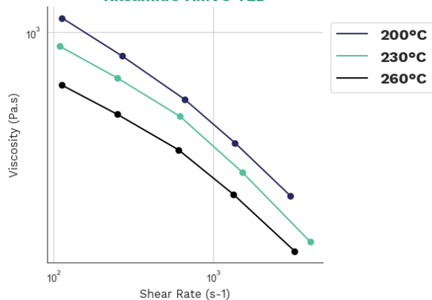
Viscosity-shear rate Rilsamid® AMVO TLD
