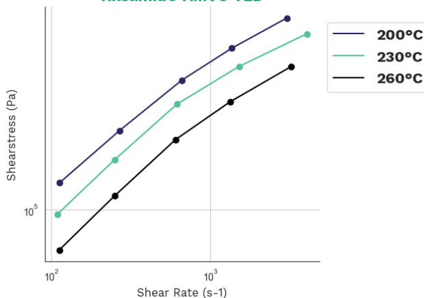
Shearstress-shear rate Rilsamid® AMVO TLD
